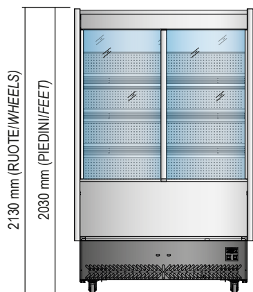
VULCANO VS - 80 - FV VS Porte scorrevoli / Sliding doors FV Frutta e Verdura Fruit and Vegetables
